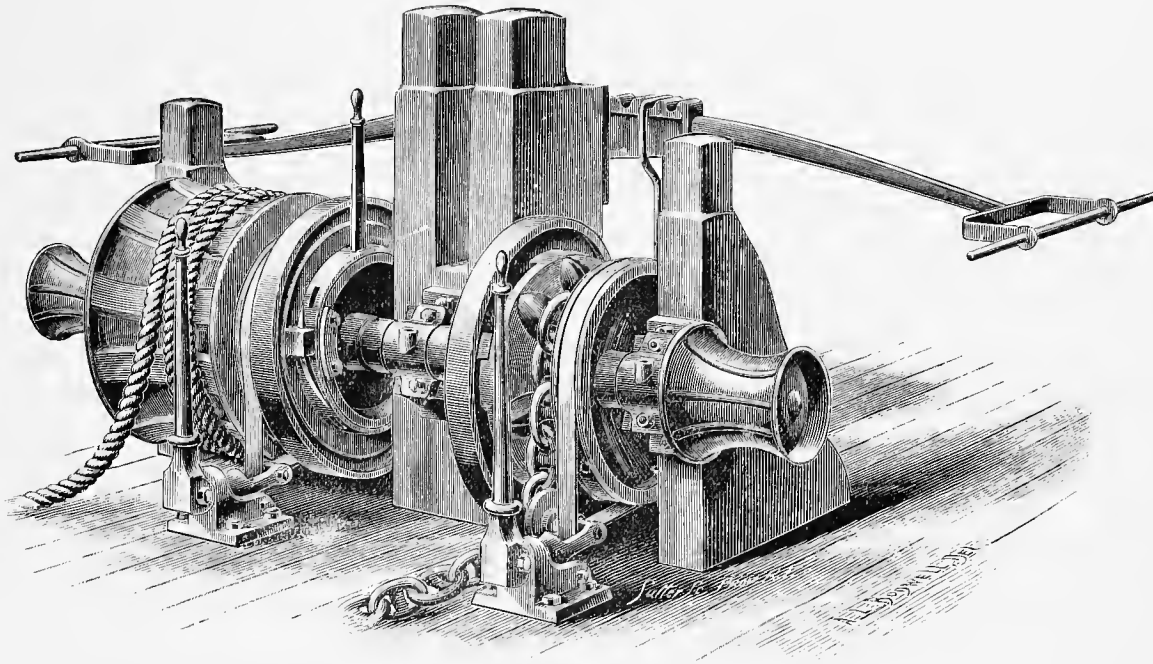
THE MANTON PATENT FISHERMAN'S WINDLASS.
